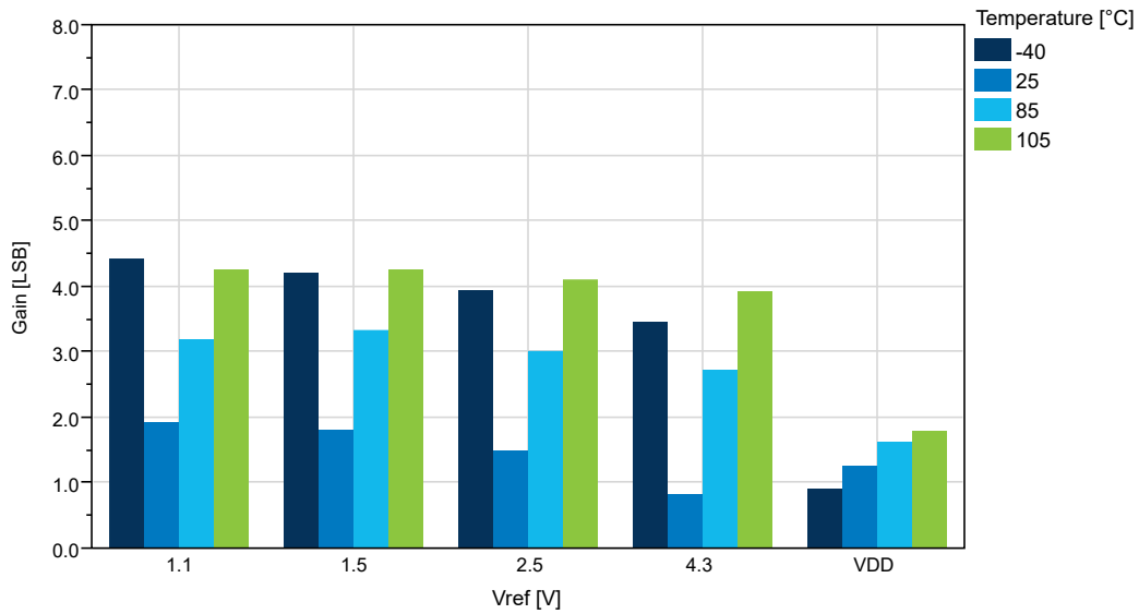
Figure 38-60. Gain Error vs. V_{ref} ( V_{DD}=5.0\text{V} , f_{ADC}=115 kps), REFSEL = Internal Reference
