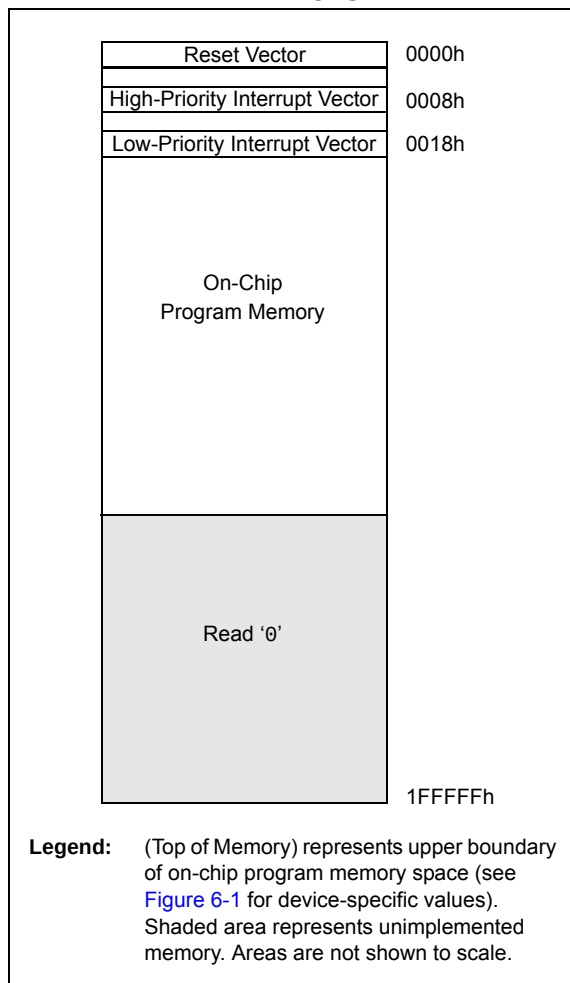
FIGURE 6-2: HARD VECTOR FOR PIC18F66K80 FAMILY DEVICES
