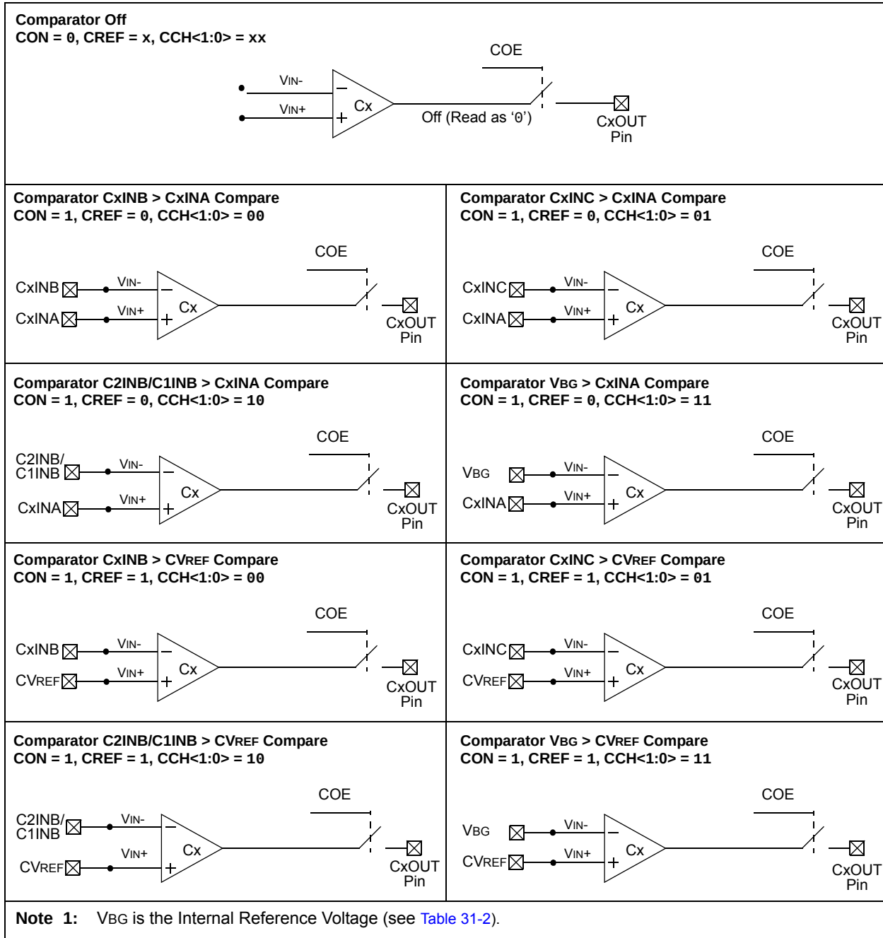
FIGURE 24-4: COMPARATOR CONFIGURATIONS
