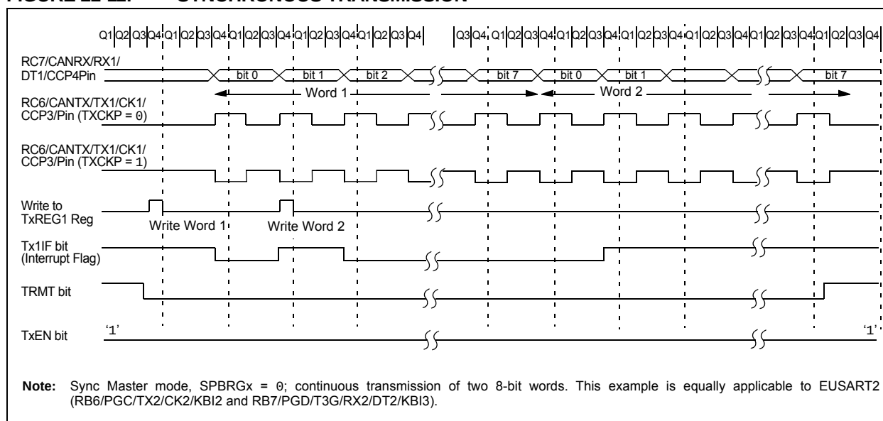
FIGURE 22-11: SYNCHRONOUS TRANSMISSION
