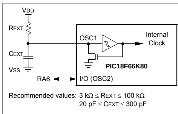
FIGURE 3-3: RCIO OSCILLATOR MODE
