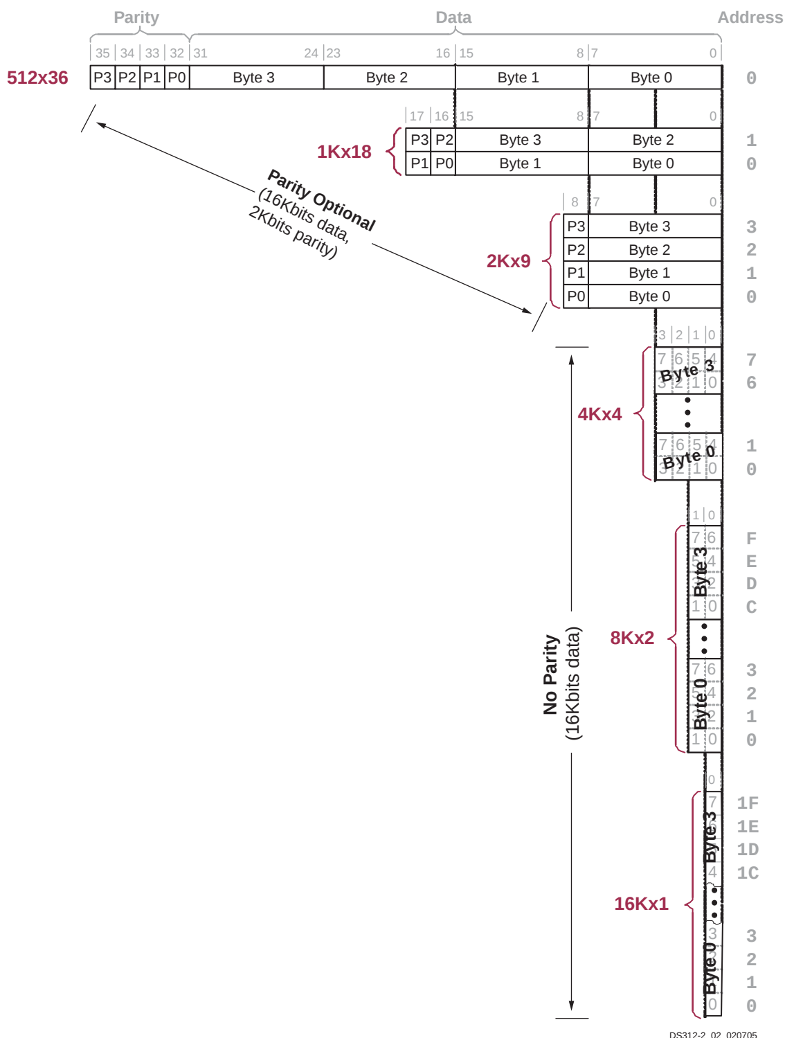
Figure 28: Data Organization and Bus-matching Operation with Different Port Widths on Port A and Port B
