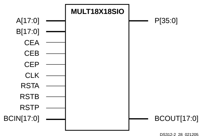
Figure 34: MULT18X18SIO Primitive
