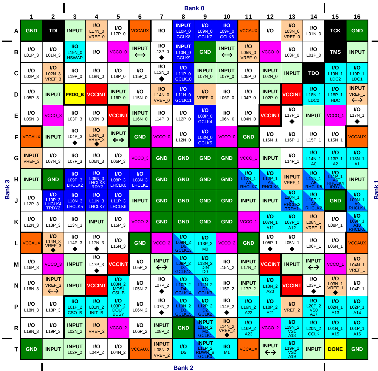
Figure 7: FT256 Package Footprint (top view)
