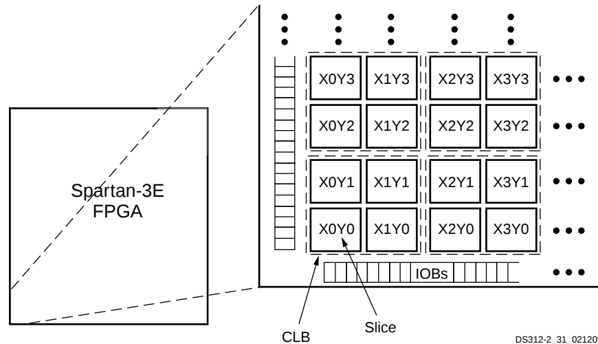
Figure 11: CLB Locations
