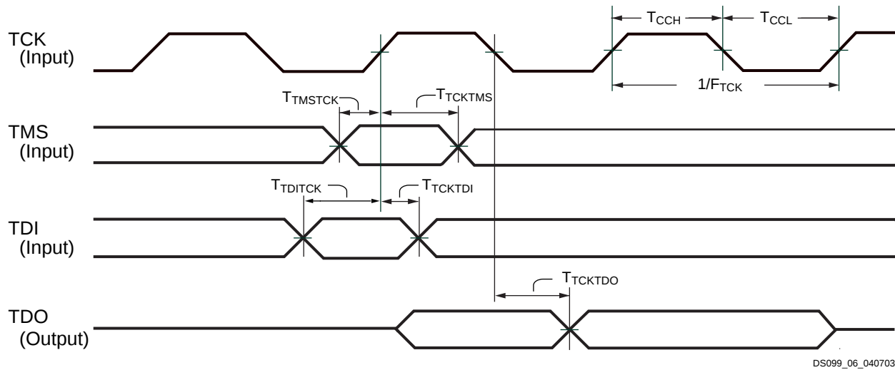
Figure 6: JTAG Waveforms
