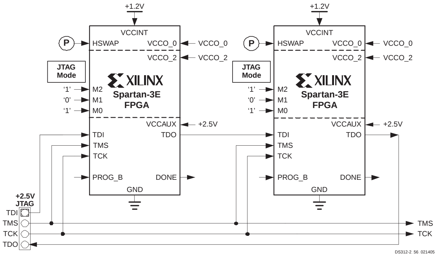
Figure 62: JTAG Configuration Mode
