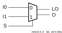
Figure 18: F5MUX with Local and General Outputs
